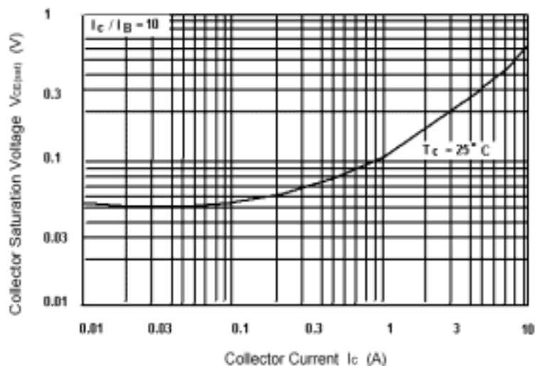
Fig.4 Collector-Emitter Saturation Voltage
