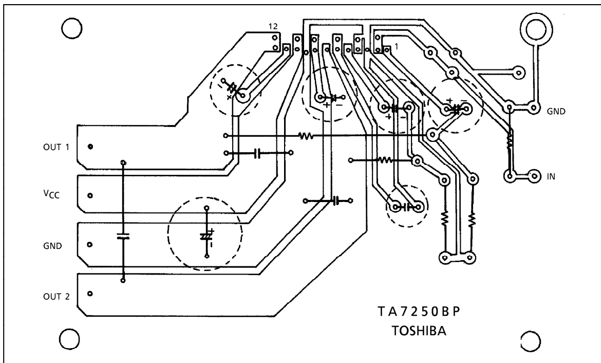
(Under view)
