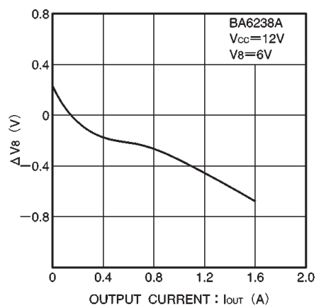
Fig.16 Pin-8 voltage variation vs. output current
