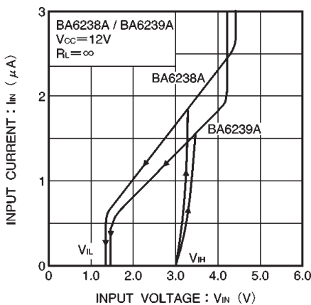
Fig.11 Input current vs. input voltage
