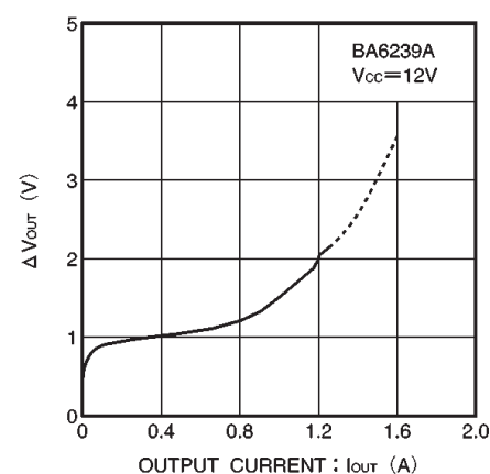
Fig.15 Output voltage variation vs. output current
