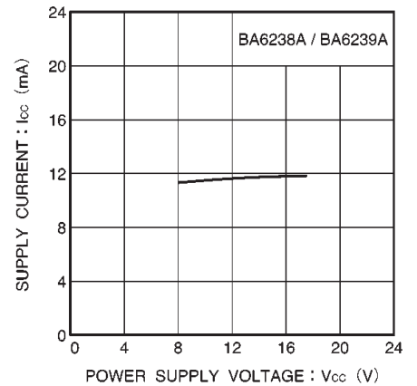
Fig.10 Supply current vs. power supply voltage
