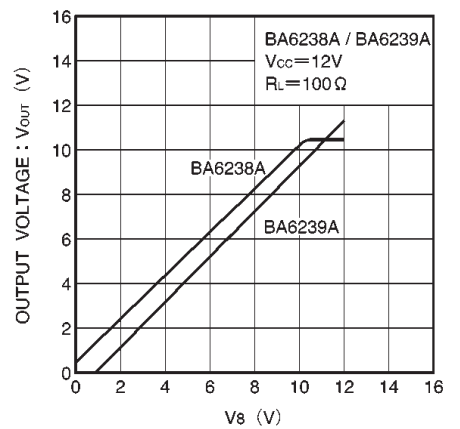
Fig.13 Output voltage vs. pin-8 voltage
