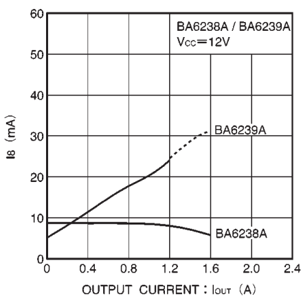
Fig.14 Pin-8 current vs. output current
