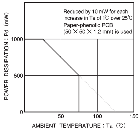
Fig.9 Power dissipation curve (BA6238AN/BA6239AN)
