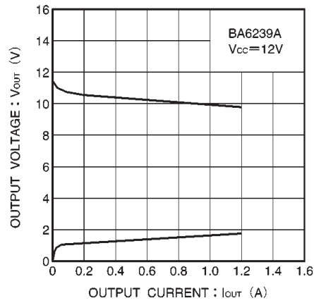
Fig.18 Output voltage vs. output current (BA6239A)
