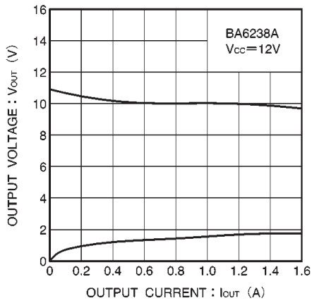
Fig.17 Output voltage vs. output current (BA6238A)
