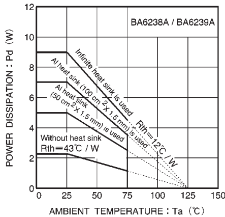
Fig.8 Power dissipation curves (BA6238A/BA6239A)
