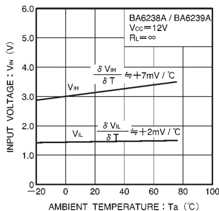
Fig.12 Input voltage vs. ambient temperature
