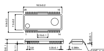
HSOP-M28
