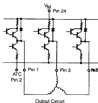
Figure 5 Output equivalent circuit
