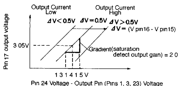
Figure 4 Motor supply voltage control
