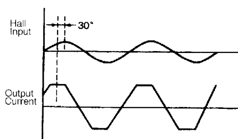
Figure 1 Hall input and output current waveforms
