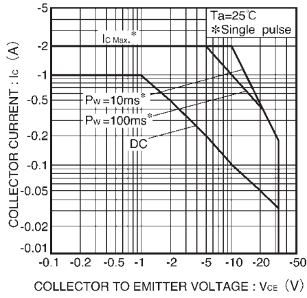
Fig.11 Safe operation area (2SB1237)
