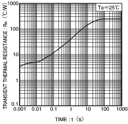
Fig.10 Transient thermal resistance (2SB1132)
