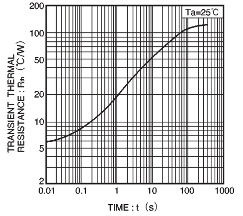
Fig.12 Transient thermal resistance (2SB1237)
