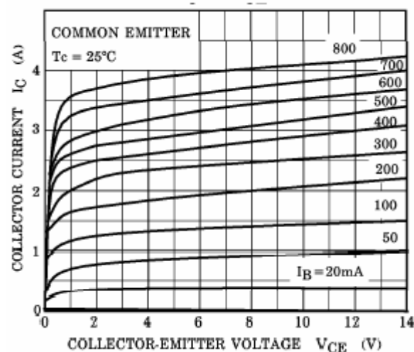
Fig.3 Static Characteristic
