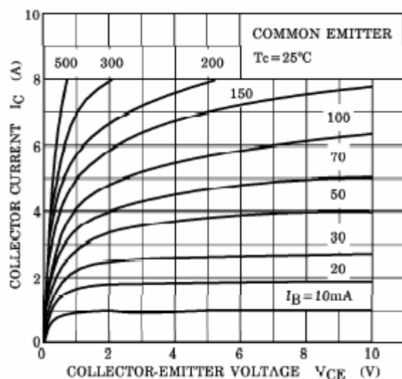
Fig.3 Static Characteristic
