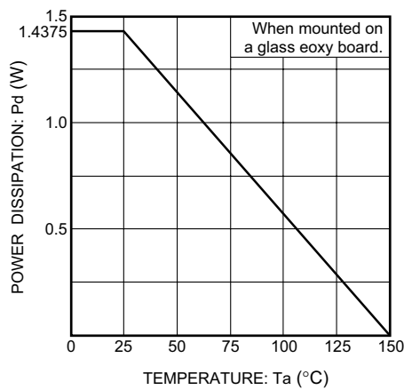
Fig. 4 Power dissipation
