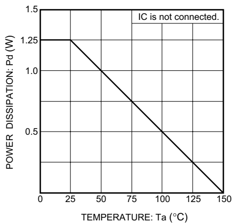
Fig. 3 Power dissipation
