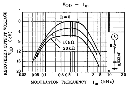
Graph 2 VOD - f_m
