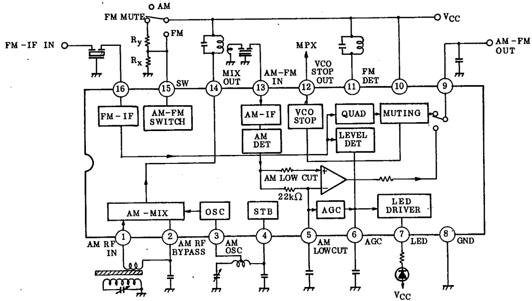
TERMINAL VOLTAGE AT NO SIGNAL ( V_{CC}=3V , T_a=25^\circ C ).
