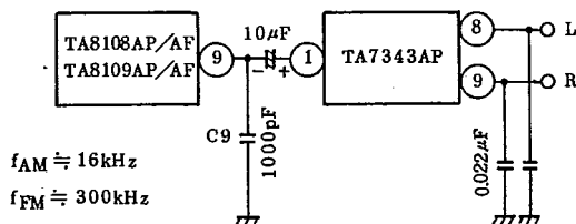
Fig. 5 CONNECTION TO TA7343AP
