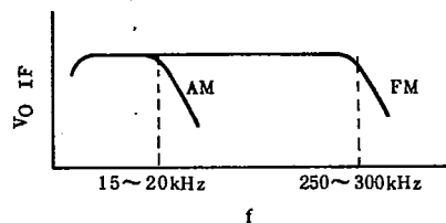
Fig. 6 FREQUENCY CHARACTERISTICS OF DET OUTPUTS
