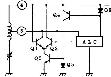
Fig.1 AM OSCILLATION CIRCUIT
