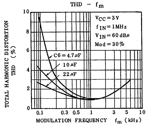
Graph 3 THD - fm
