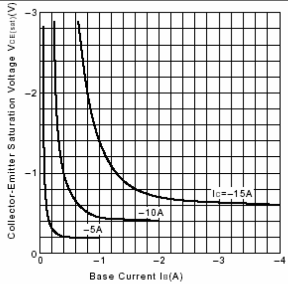
Fig.4 V_{CE(sat)}-I_B Characteristics
