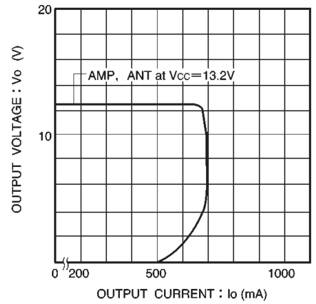
Fig.7 Output voltage vs. current
