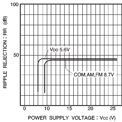
Fig.8 Ripple rejection vs. power supply voltage
