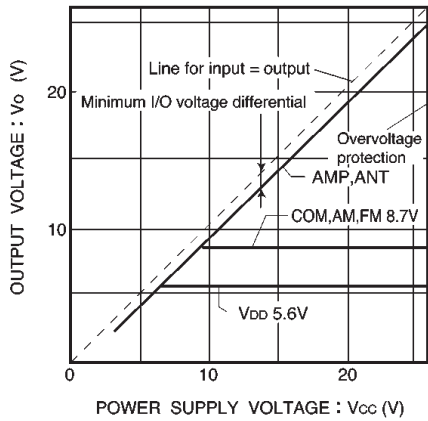
Fig.5 Output voltage vs. power supply voltage
