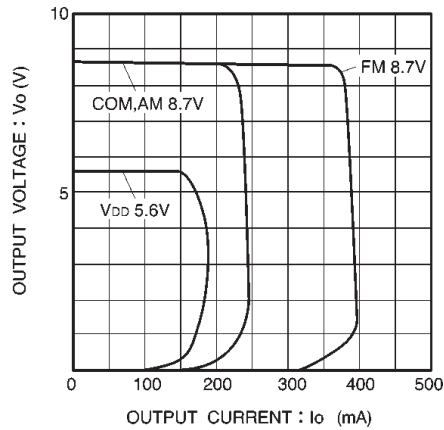
Fig.6 Output voltage vs. current
