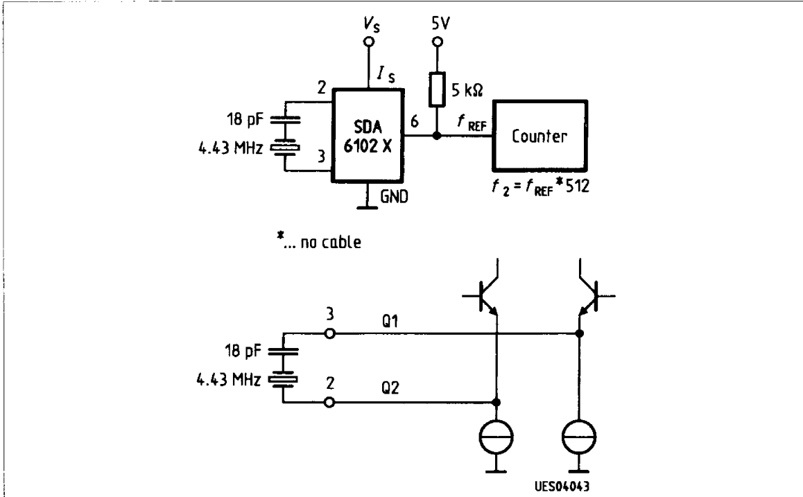
Test Circuit 1
