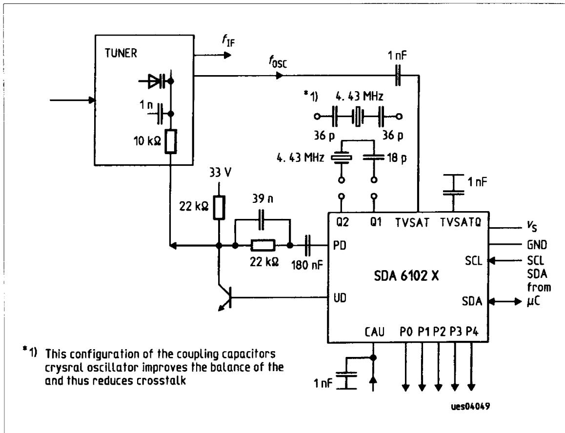
Application Circuit
