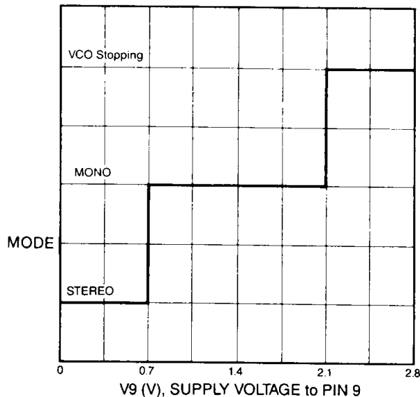
SCHMATIC DIAGRAM of PIN 9 CONTROL
