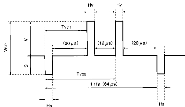
Fig. 2 Output waveform
