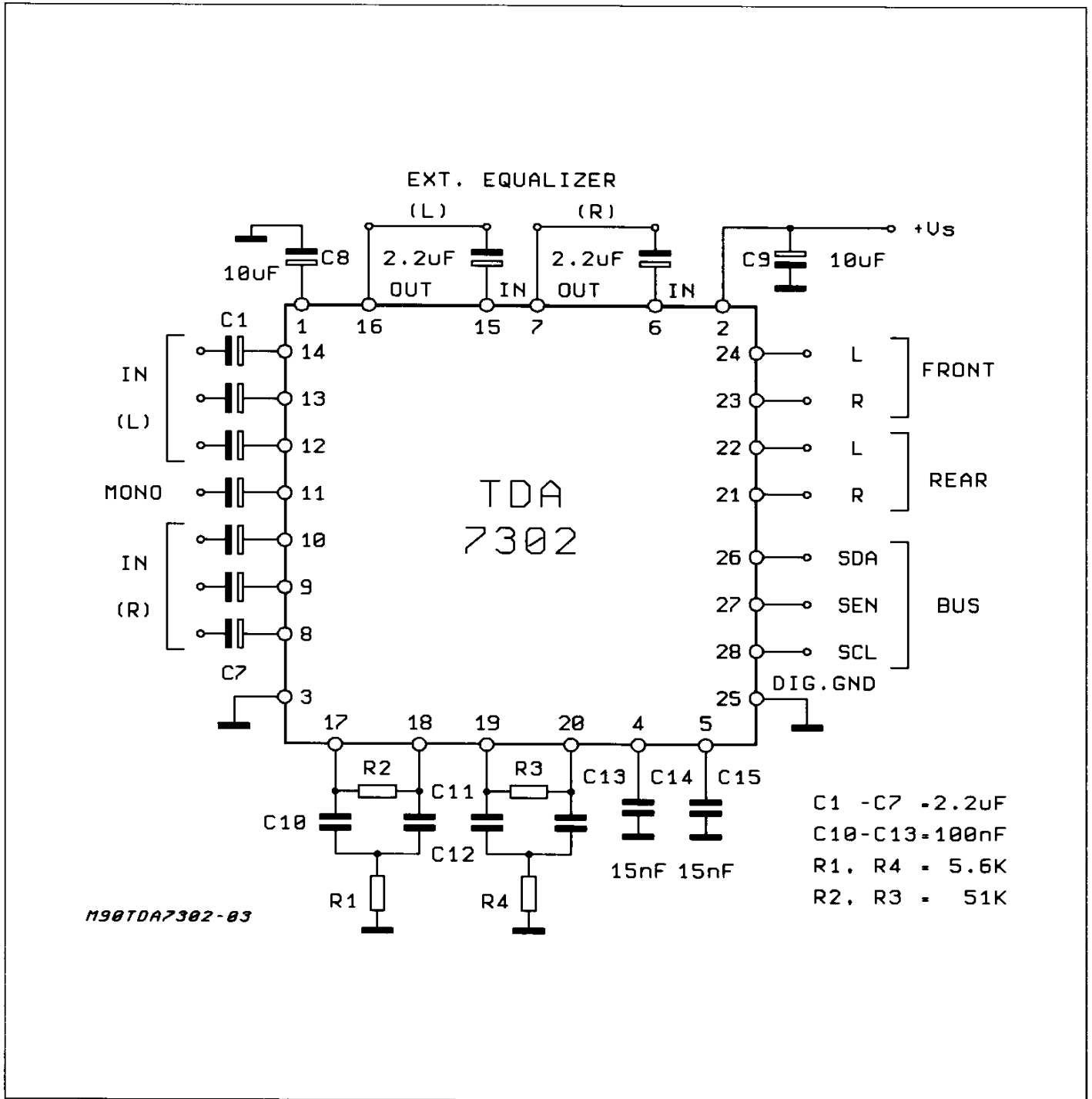
Figure 1: Application Circuit
