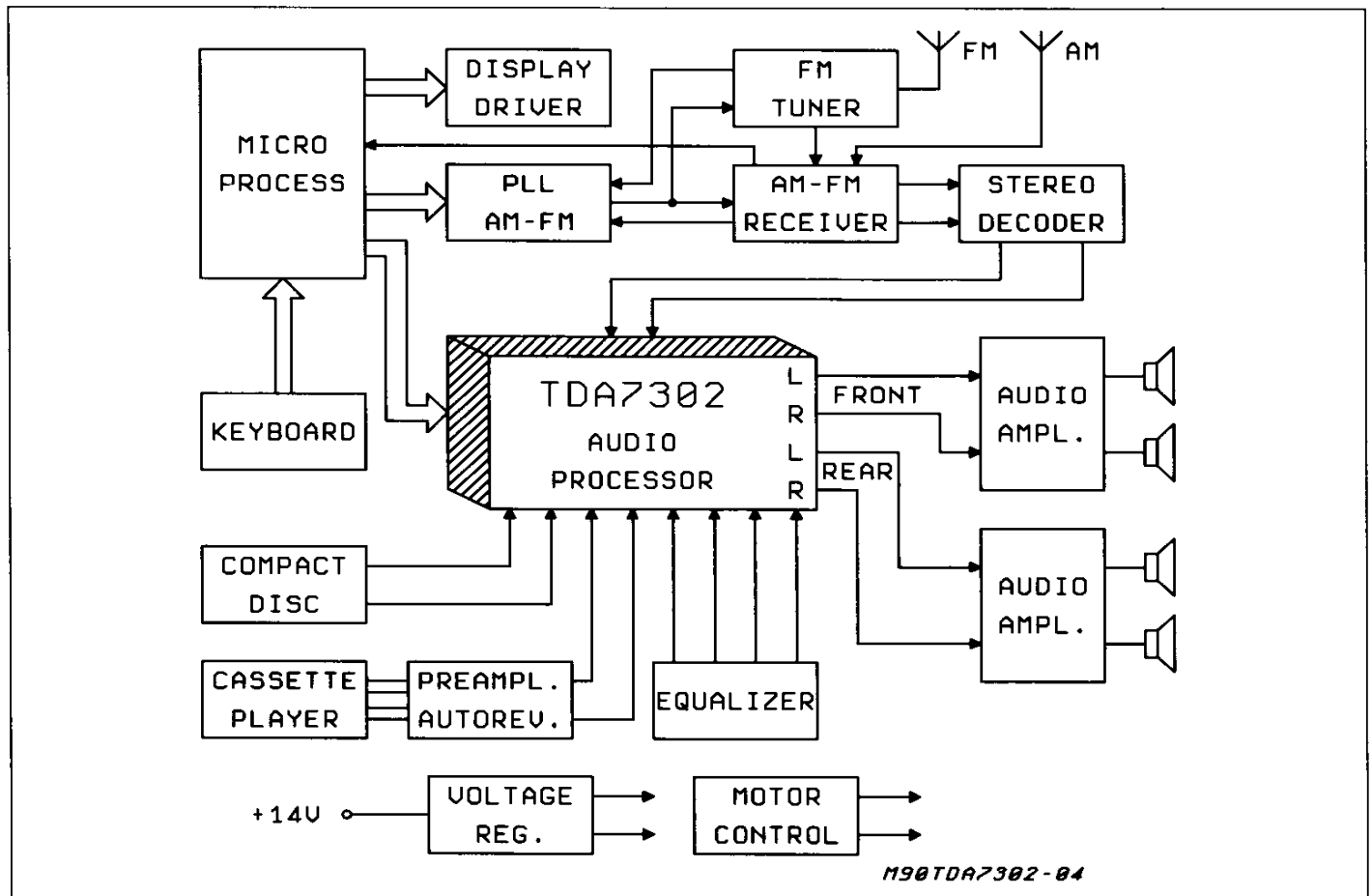
Figure 15: Complete Car-Radio System using Digital Controlled Audio Processor
