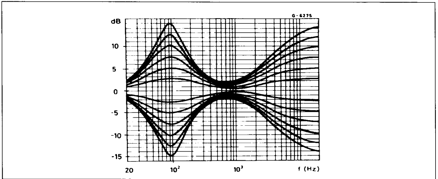
Figure 14: Typical Tone Response
