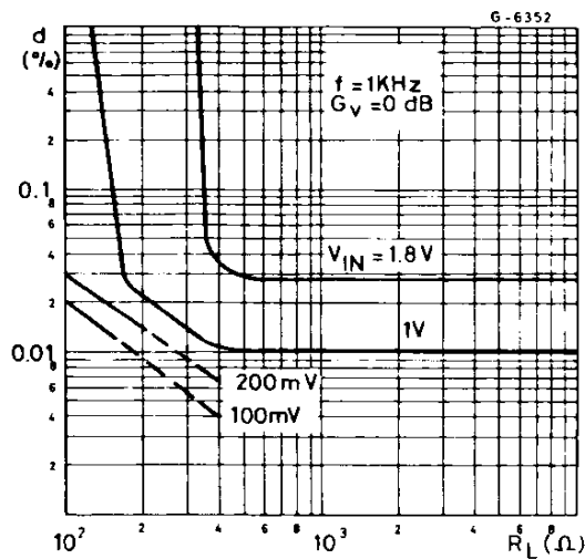
Figure 7: Distortion vs. Load Resistance
