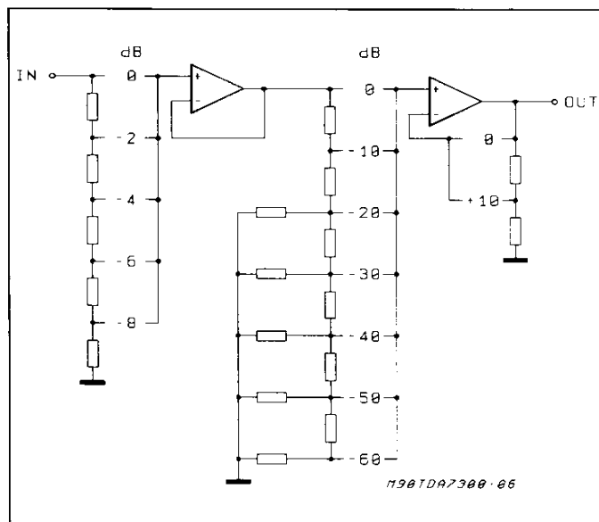
Figure 12: Volume Control
