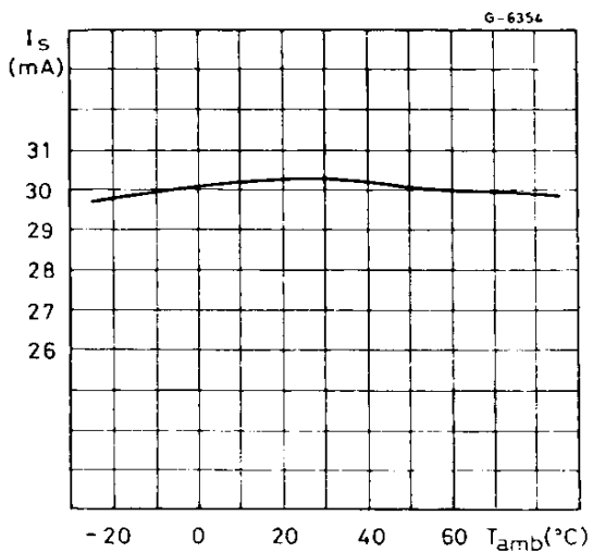
Figure 11: Quiescent Current vs. Temperature
