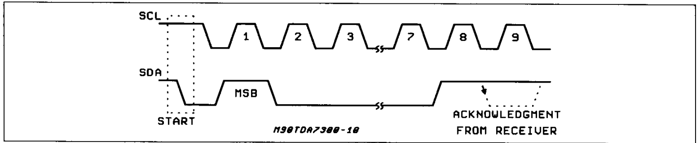
Figure 18: Acknowledge on the I 2 CBUS
