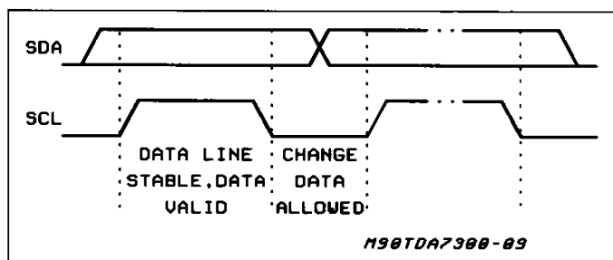
Figure 16: Data Validity on the I 2 C BUS
