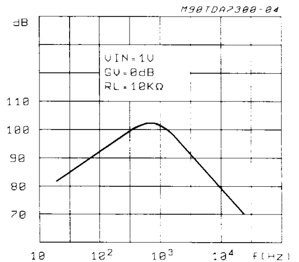
Figure 8: Channel Separation (L1 - R1) vs. Frequency
