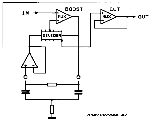
Figure 13: Bass Control
