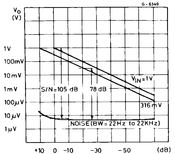
Figure 4: Signal to Noise Ratio vs. Volume Setting
