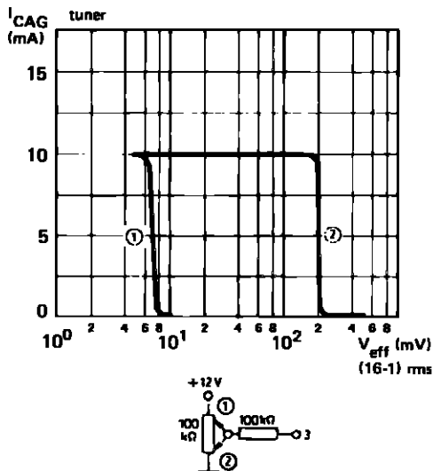
Figure 7 : AGC Tuner Current Curve
