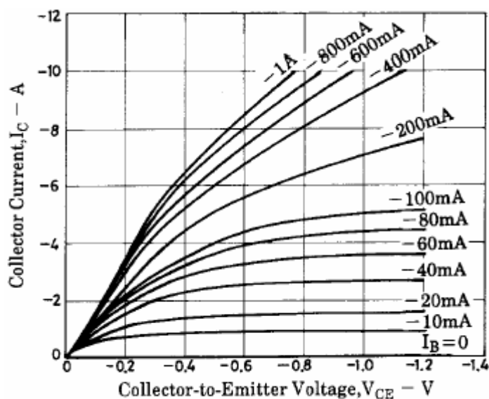
Fig.3 Static Characteristic
