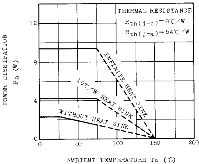
P_D - T_a TA7245BP, CP, BP(LB)
