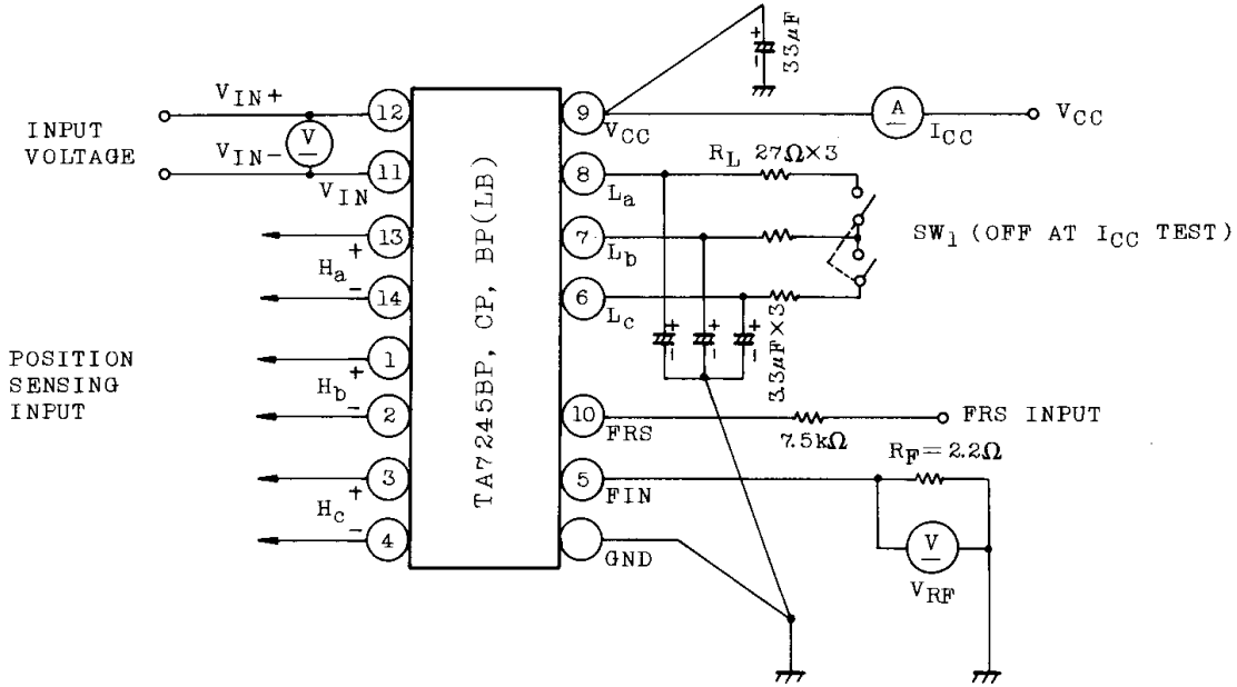
TEST CIRCUIT 1
