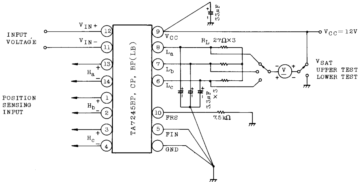
TEST CIRCUIT 2
