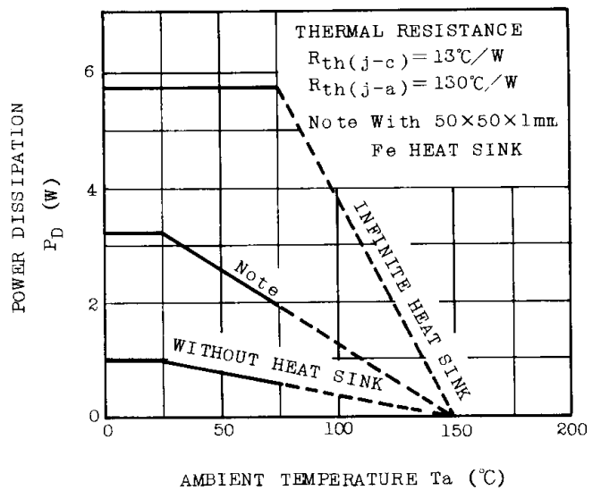
P_D - T_a TA7245F
