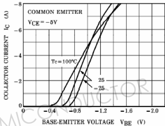
Fig.6 Base-Emitter On Voltage
